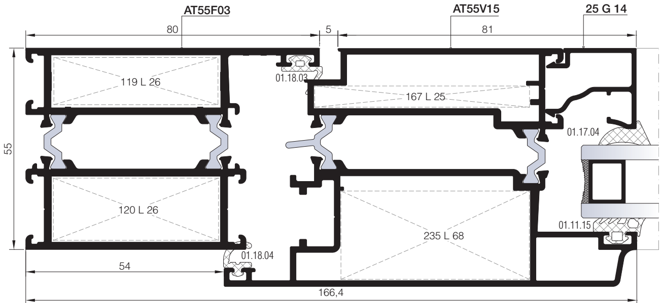
(38A) DETAYI DETAIL
